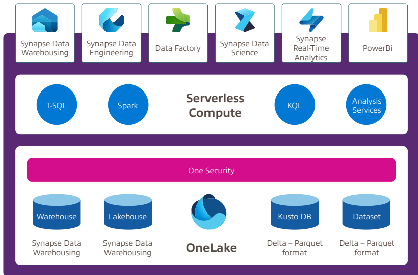
Figure 1: Microsoft Fabric overview
